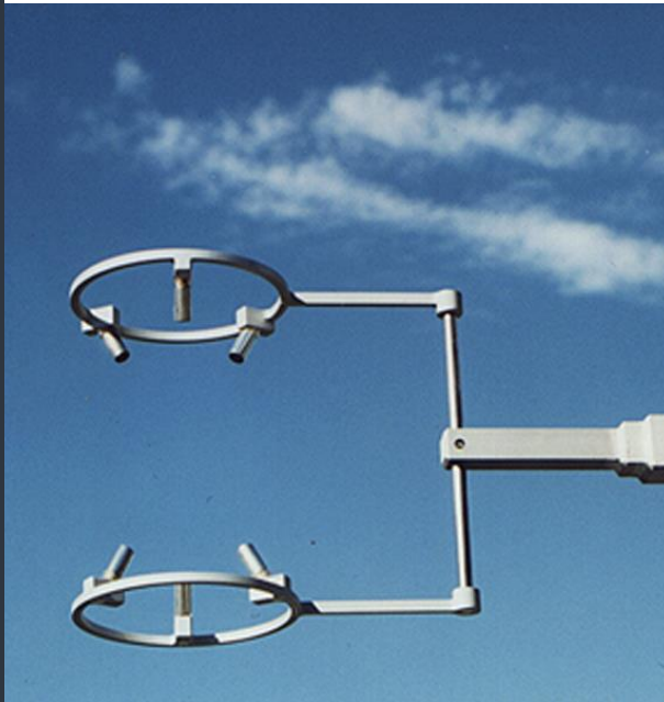
A non-orthogonal design for applications that require a high range of velocity.
